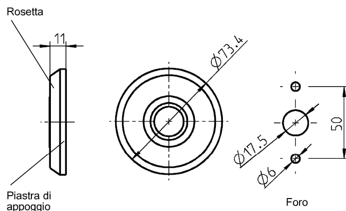
Rosetta in poliammide GF nera
